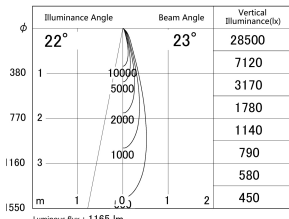
■ Direct Horizontal Illuminance DD155-1025MW9030
