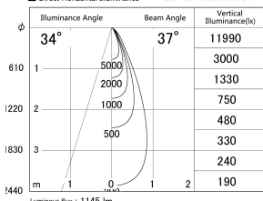
■ Direct Horizontal Illuminance DD155-1035MW9030
