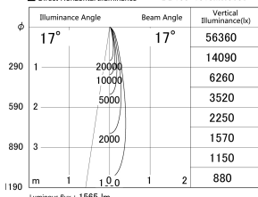
■ Direct Horizontal Illuminance DD155-1515MW9030
