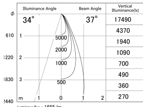
■ Direct Horizontal Illuminance DD155-1535MW9030
