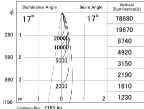
■ Direct Horizontal Illuminance DD155-2015MW9030
