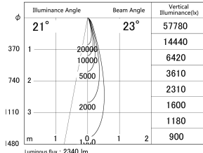
■ Direct Horizontal Illuminance DD155-2025MW9030
