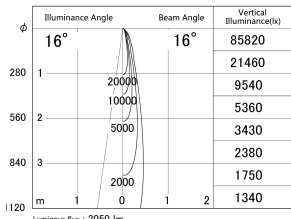
■ Direct Horizontal Illuminance DD155-2515MW9030
