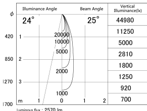
■ Direct Horizontal Illuminance DD155-2525MW9030
