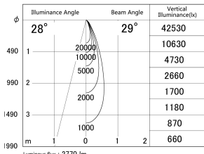
■ Direct Horizontal Illuminance DD155-2530MW9030
