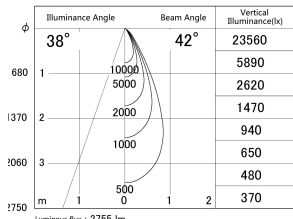
■ Direct Horizontal Illuminance DD155-2540MW9030
