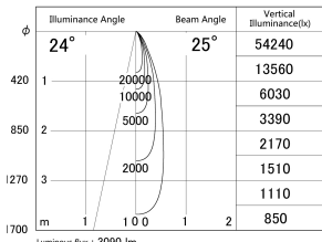
■ Direct Horizontal Illuminance DD155-3025MW9030
