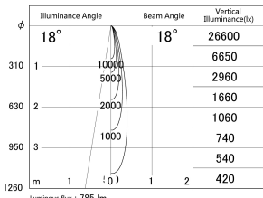
■ Direct Horizontal Illuminance DD155-0815MW9035
