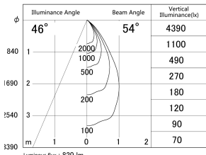
■ Direct Horizontal Illuminance DD155-0855MW9035
