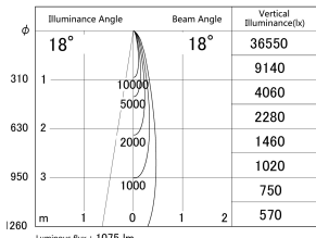
■ Direct Horizontal Illuminance DD155-1015MW9035
