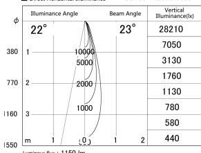
■ Direct Horizontal Illuminance DD155-1025MW9035
