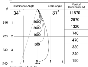
■ Direct Horizontal Illuminance DD155-1035MW9035
