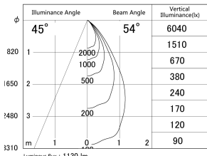
■ Direct Horizontal Illuminance DD155-1055MW9035
