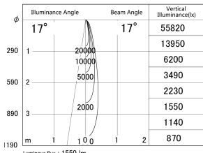
■ Direct Horizontal Illuminance DD155-1515MW9035
