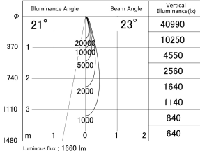
■ Direct Horizontal Illuminance DD155-1525MW9035
