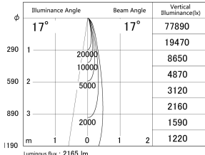
■ Direct Horizontal Illuminance DD155-2015MW9035
