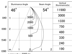
■ Direct Horizontal Illuminance DD155-2055MW9035
