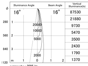
■ Direct Horizontal Illuminance DD155-2515MW9035
