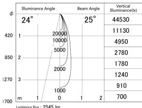
■ Direct Horizontal Illuminance DD155-2525MW9035
