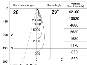
■ Direct Horizontal Illuminance DD155-2530MW9035
