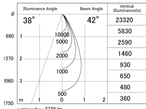
■ Direct Horizontal Illuminance DD155-2540MW9035
