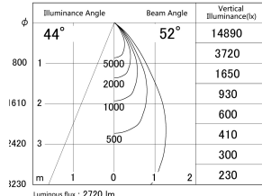
■ Direct Horizontal Illuminance DD155-2555MW9035
