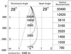
■ Direct Horizontal Illuminance DD155-3030MW9035
