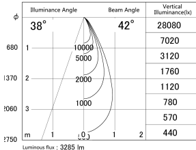
■ Direct Horizontal Illuminance DD155-3040MW9035
