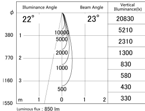
■ Direct Horizontal Illuminance DD155-0825MW9040
