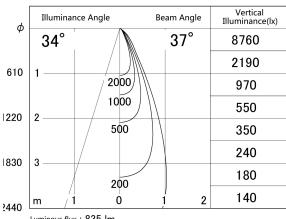
■ Direct Horizontal Illuminance DD155-0835MW9040
