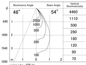
■ Direct Horizontal Illuminance DD155-0855MW9040
