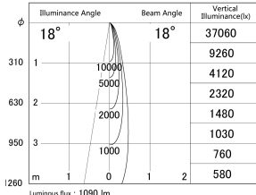
■ Direct Horizontal Illuminance DD155-1015MW9040
