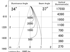
■ Direct Horizontal Illuminance DD155-1535MW9040
