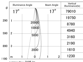
■ Direct Horizontal Illuminance DD155-2015MW9040
