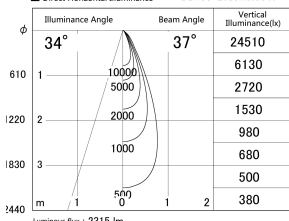
■ Direct Horizontal Illuminance DD155-2035MW9040
