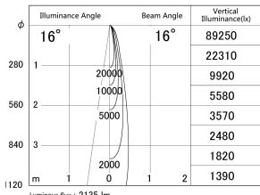
■ Direct Horizontal Illuminance DD155-2515MW9040
