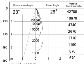
■ Direct Horizontal Illuminance DD155-2530MW9040
