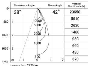
■ Direct Horizontal Illuminance DD155-2540MW9040
