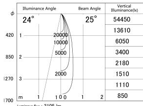
■ Direct Horizontal Illuminance DD155-3025MW9040
