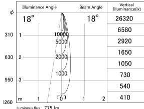
■ Direct Horizontal Illuminance DD155-0815MB9027
