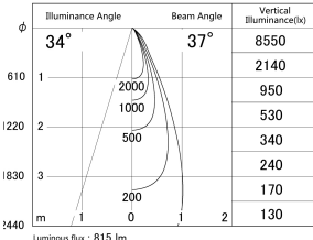
■ Direct Horizontal Illuminance DD155-0835MB9027
