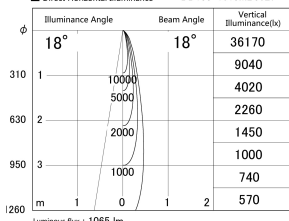
■ Direct Horizontal Illuminance DD155-1015MB9027
