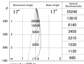
■ Direct Horizontal Illuminance DD155-1515MB9027
