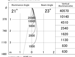
■ Direct Horizontal Illuminance DD155-1525MB9027
