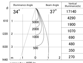
■ Direct Horizontal Illuminance DD155-1535MB9027
