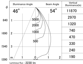
■ Direct Horizontal Illuminance DD155-2055MB9027
