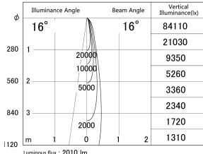
■ Direct Horizontal Illuminance DD155-2515MB9027
