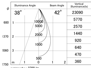
■ Direct Horizontal Illuminance DD155-2540MB9027
