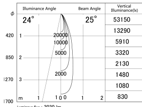
■ Direct Horizontal Illuminance DD155-3025MB9027
