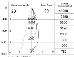
■ Direct Horizontal Illuminance DD155-3030MB9027
